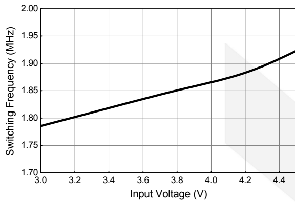
Switching Frequency vs. Input Voltage
